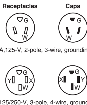
FIGURE 552.44(C)(1) Attachment Cap and Receptacle Configurations.
